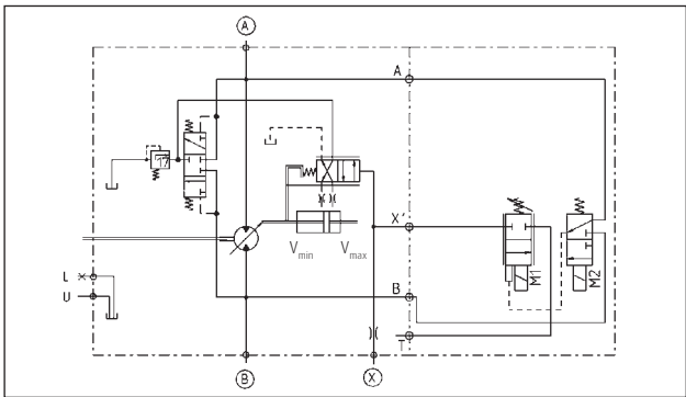
EH1P. Case pressure as reference, «Bleed» regulation
