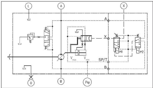
EH1P-CA. Feed pressure as reference, «Non-Bleed» regulation
